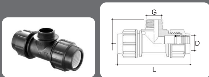
MALE TEE (M.T.) *BSP TAPER MALE THREADED. 外牙梯
