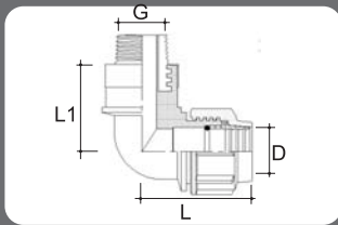
PP MALE ELBOW C/W BRASS THREADED INSERT (COMPRESSION TYPE)
