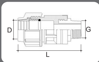
PP MALE ADAPTOR C/W BRASS THREADED INSERT (COMPRESSION TYPE)
