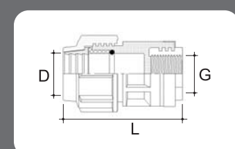
PP FEMALE ADAPTOR C/W BRASS THREADED INSERT (COMPRESSION TYPE)
