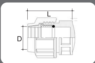
COMPRESSION END CAP (E.C) 元帽
