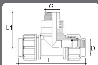
PP MALE TEE C/W BRASS THREADED INSERT (COMPRESSION TYPE)
