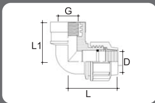
PP FEMALE ELBOW C/W BRASS THREADED INSERT (COMPRESSION TYPE)
