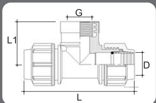
PP FEMALE TEE C/W BRASS THREADED INSERT (COMPRESSION TYPE)
