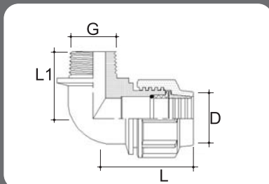
MALE ELBOW (M.E.) *BSP TAPER MALE THREADED. 外牙彎頭
